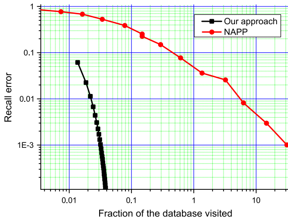
Fig. 7. Average fraction of visited elements within a single k-NN-search vs recall error for 10 million CoPHiR objects.
