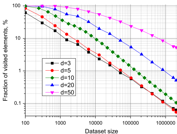
Fig. 3. Average fraction of visited elements within a single 10-NN-search with 0.999 recall versus the size of the dataset for different dimensionality.
